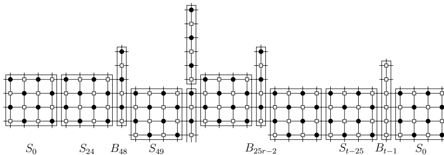
Figure 3: Distance graph D(1, t) for even t .
