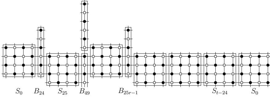
Figure 2: Distance graph D(1, t) for odd t .
