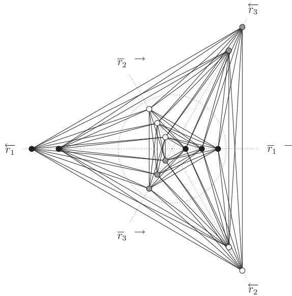
FIGURE 1. An alternating 3-line drawing of K_{5,5,5} with 192 crossings. Points on opposite rays are in one partite set. The partite sets are distinguished by the color of the nodes. The distances were slightly adjusted for visual clarity. The rays and unit circle are shown faint and dotted.
